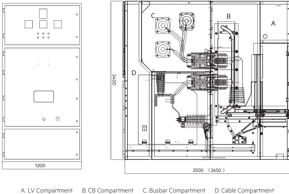
SecoGear cross section view
