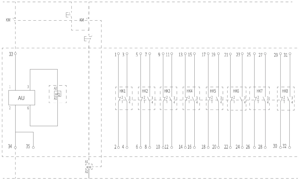
The schematic shows the following state: The contactor is switched on
