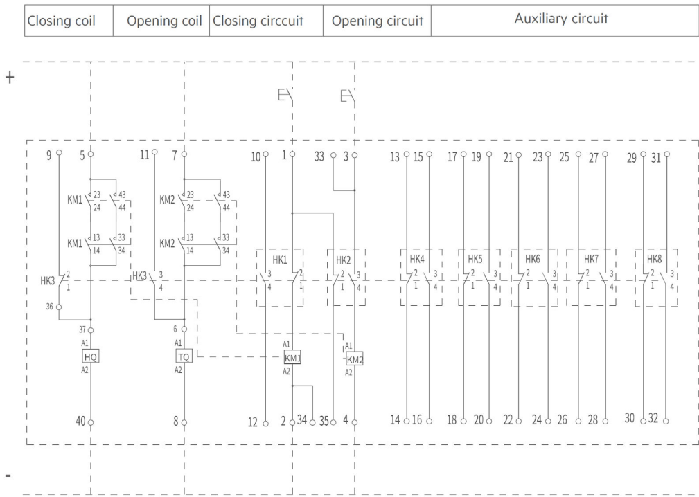
The schematic shows the following state: The contactor is switched on
