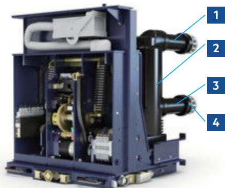
Figure 2. Primary circuit
